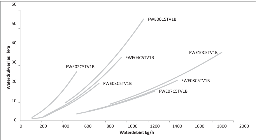
Waterdrukverlies curve 3-Rijen Convector unit
