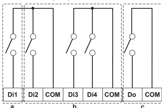
Schematic wiring diagram with Di and Do terminals
